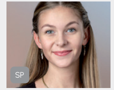
Samira Martini
